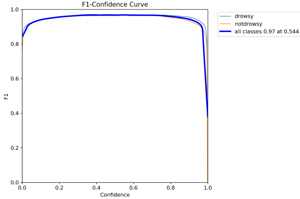
Figure: 5. F1-Score
